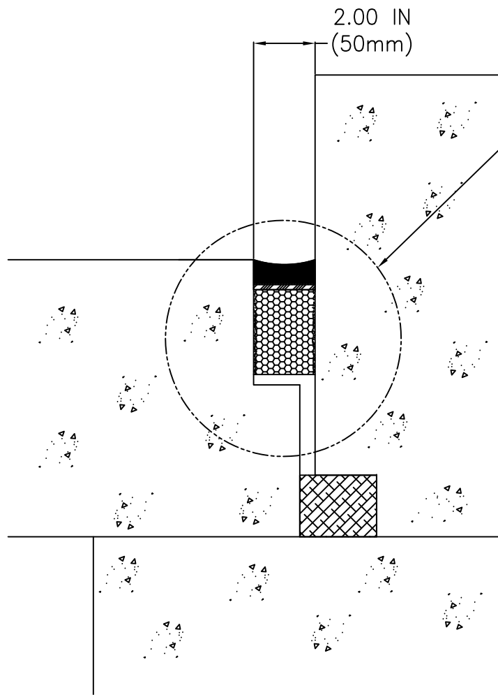
JOINT @ "Y"
