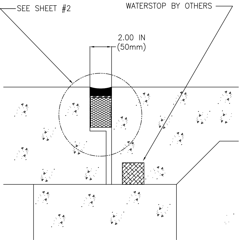
JOINT @ "CL"
