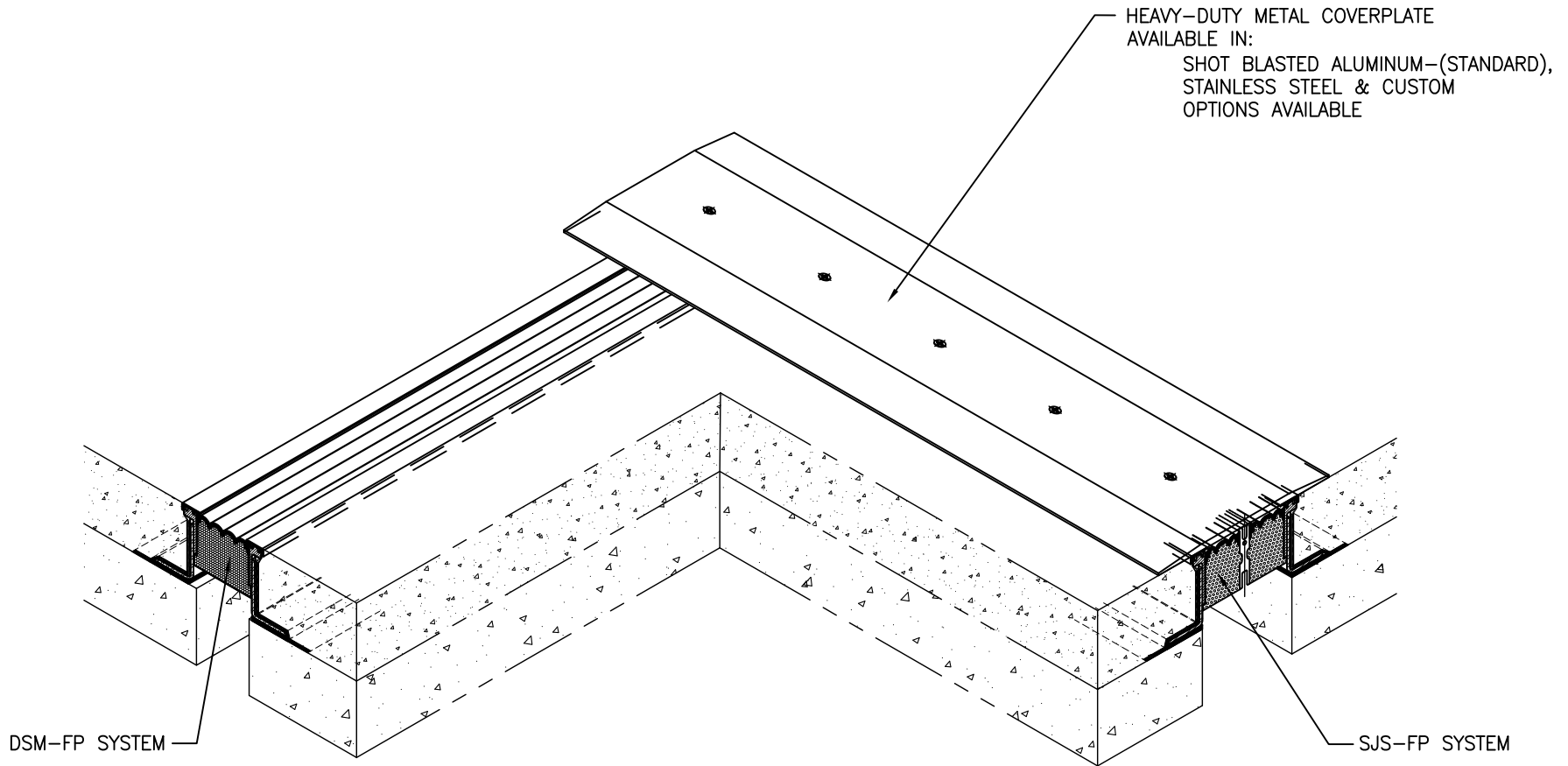
SYSTEMS SHOWN - DSM-FP-400-115-DD WITH A HORIZONTAL 90 DEG TRANSITION TO SJS-FP-600-115-DD
