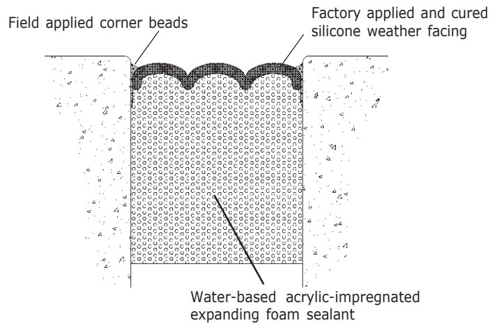
COLORSEAL with silicone corner beads in a typical installation. Corner beads shown may be dispensed with in certain applications.
