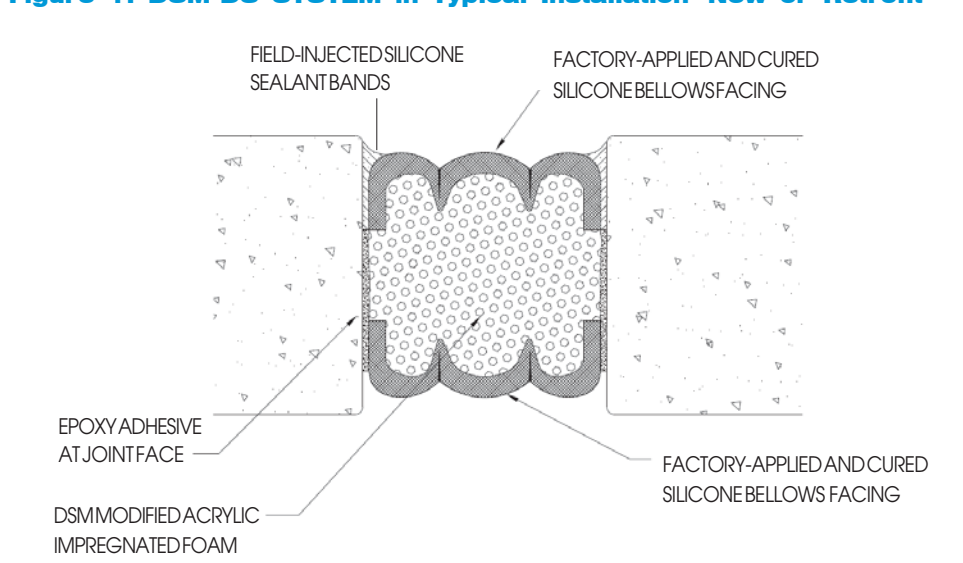
Figure 1: DSM-DS SYSTEM in Typical Installation--New or Retrofit
