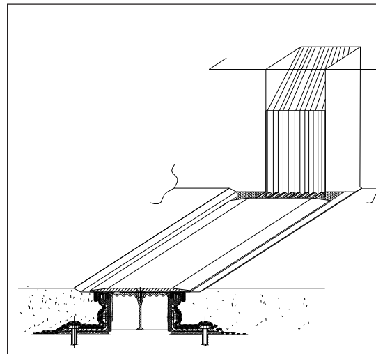
FIGURE 2: Continuity of Seal
